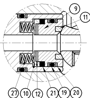
SEAT DETAILS
