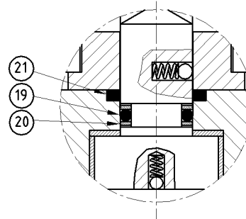
STEM DETAILS
