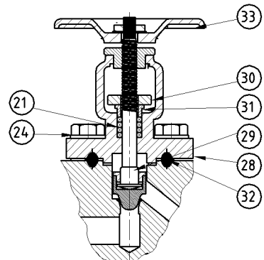
BLEED NEEDLE VALVE DETAIL
