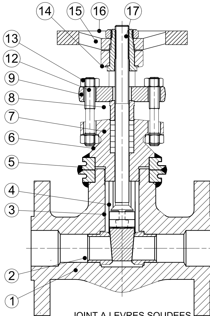
JOINT A LEVRES SOUDEES SEALED LIPS JOINT TYPE
